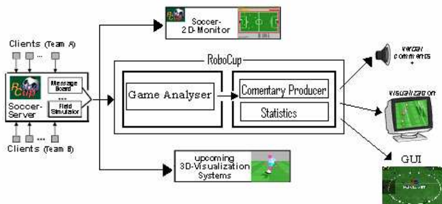
Connecting Soccer Server and Our system
